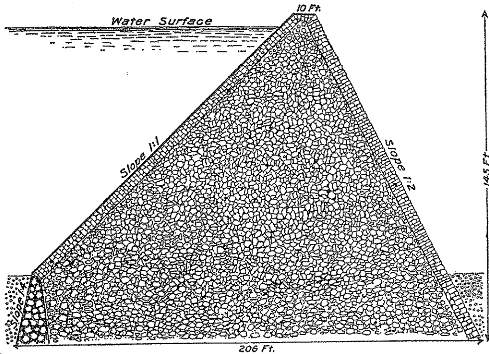
FIG. 14.—Profile of Queen Creek dam.
