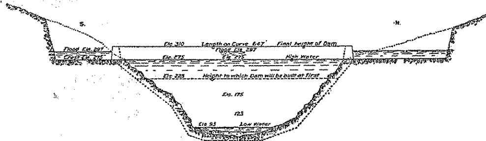
FIG. 9.—Elevation of proposed dam on Salt River.
