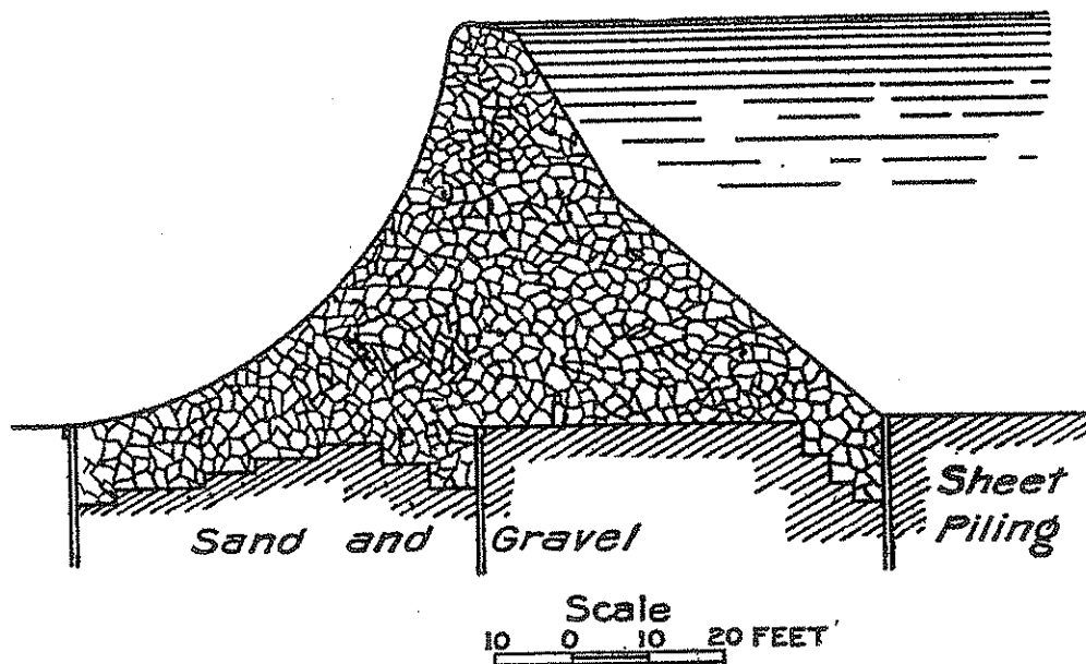
FIG. 15.—Section of proposed South Gila dam.
