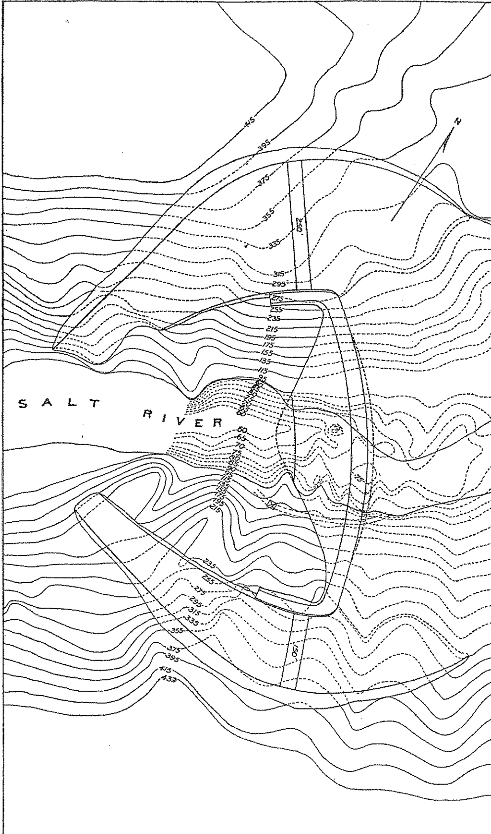
PLAN OF PROPOSED DAM ON SALT RIVER, SHOWING SPILLWAYS.
