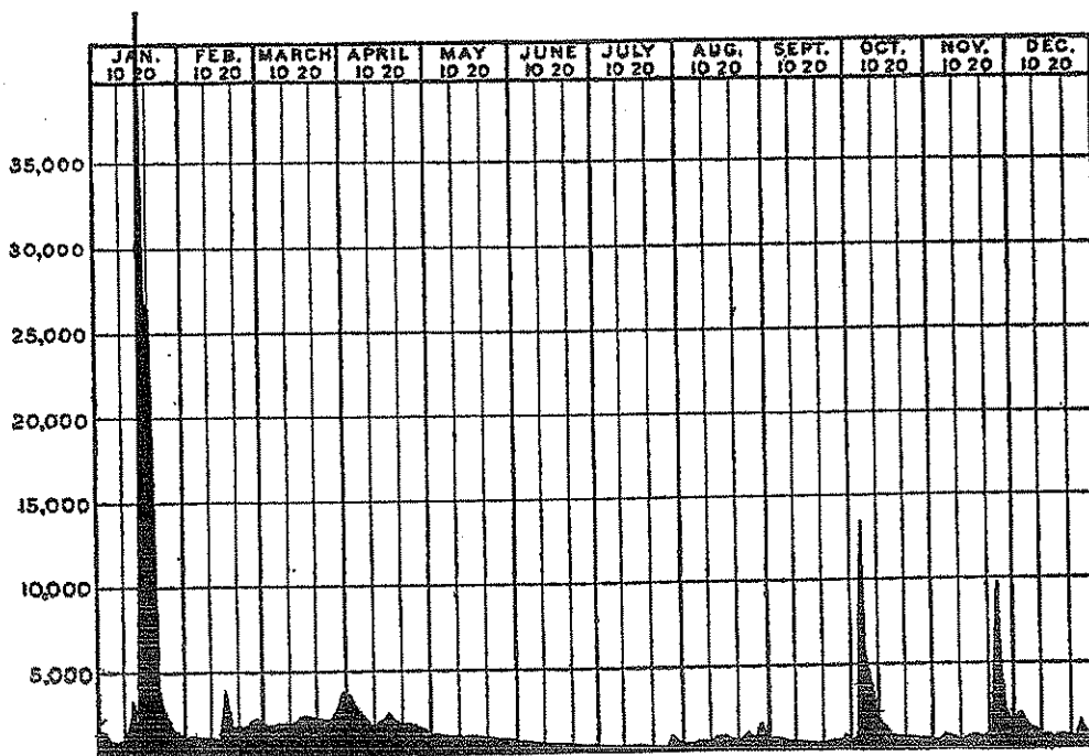
FIG. 5.—Daily discharge of Salt River above Verde, 1895.
