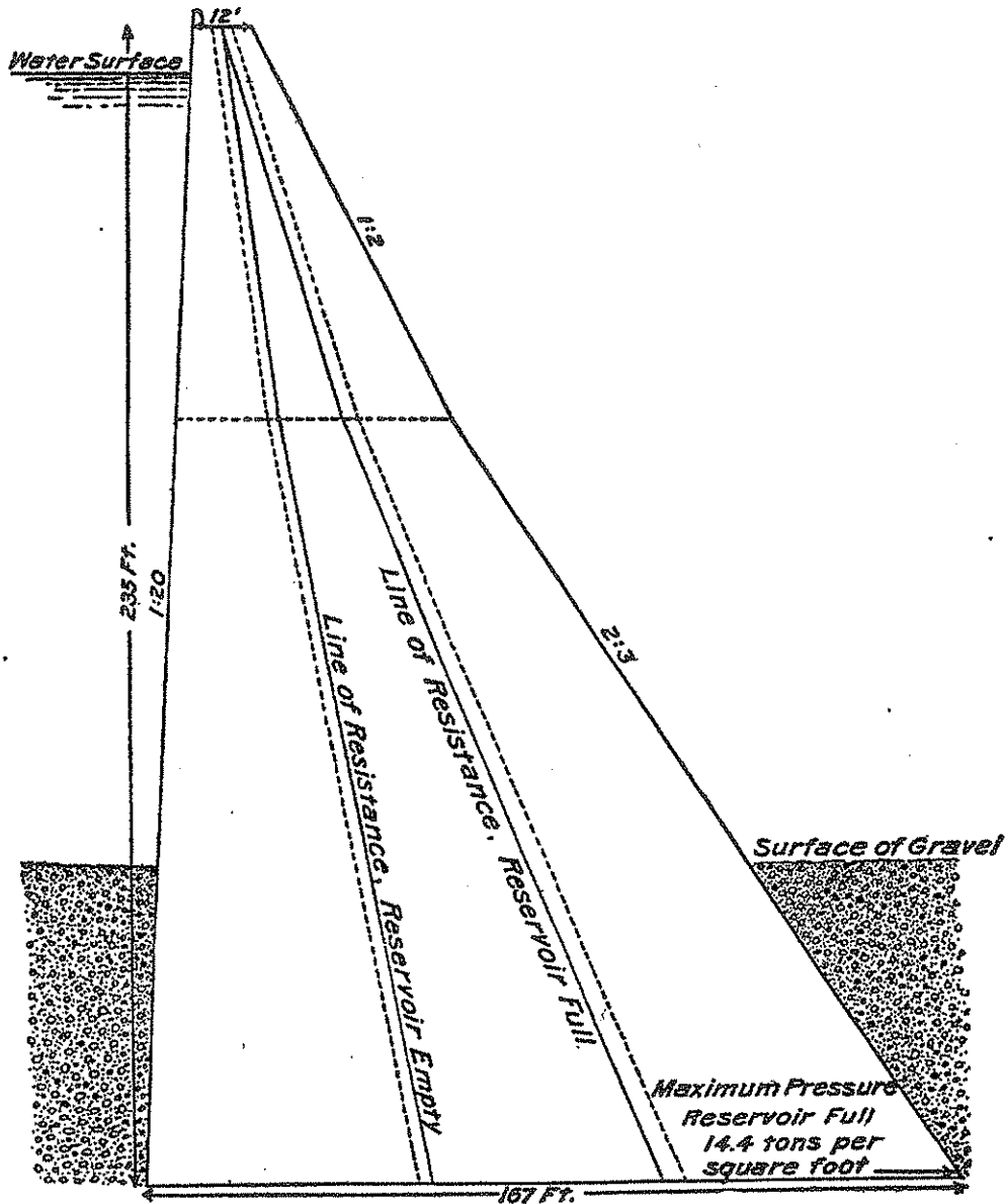
FIG. 13.—Profile of proposed dam at The Buttes.
