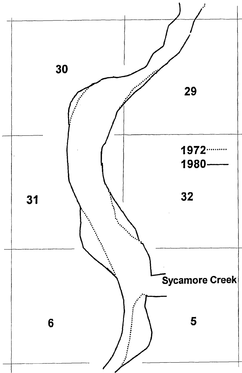
Figure 5c. Changes in the position and width of the flood channel of the lower Verde River near Sycamore Creek between 1972 and 1980.
