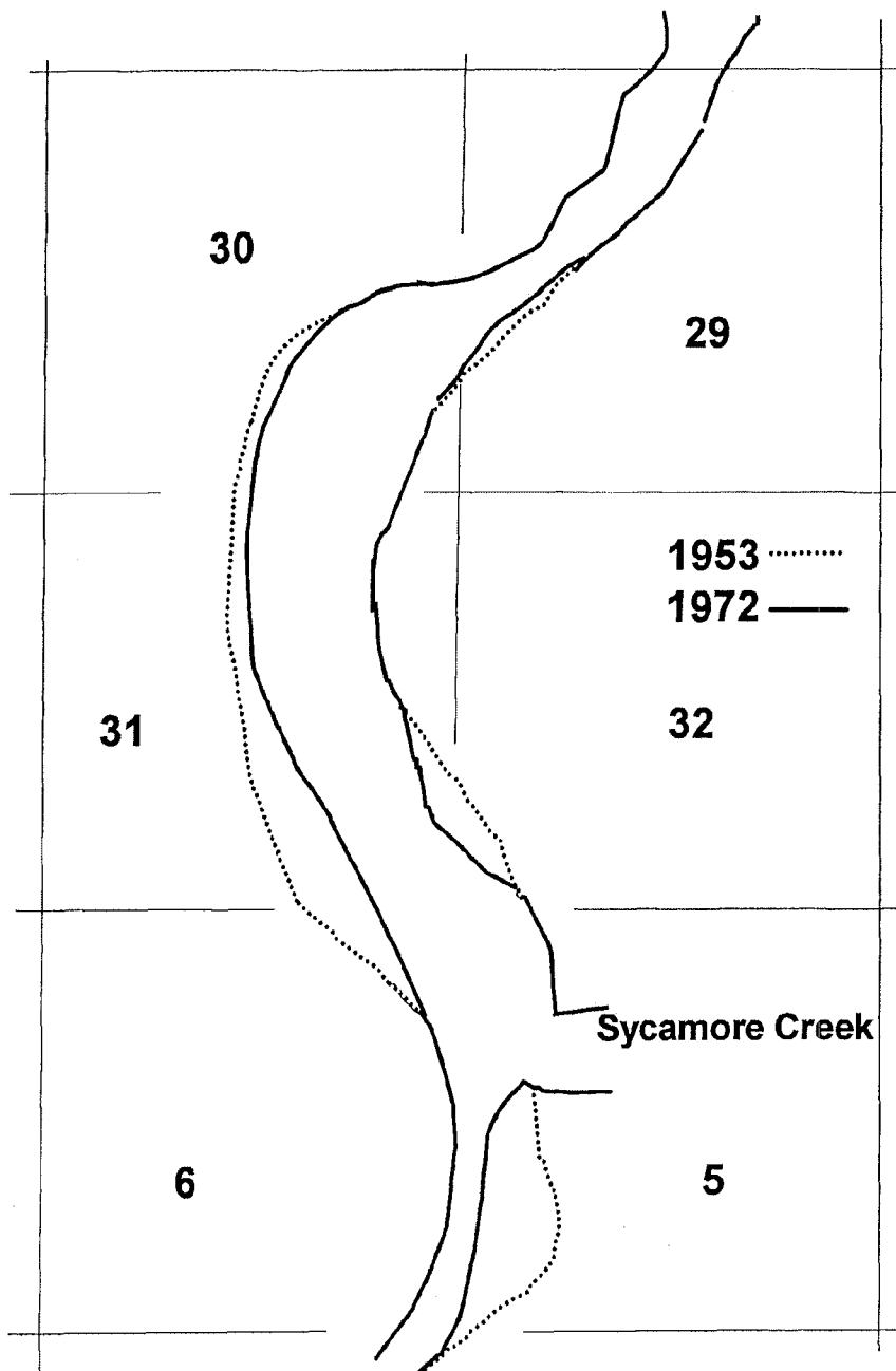
Figure 5b. Changes in the position and width of the flood channel of the lower Verde River near Sycamore Creek between 1953 and 1972.
