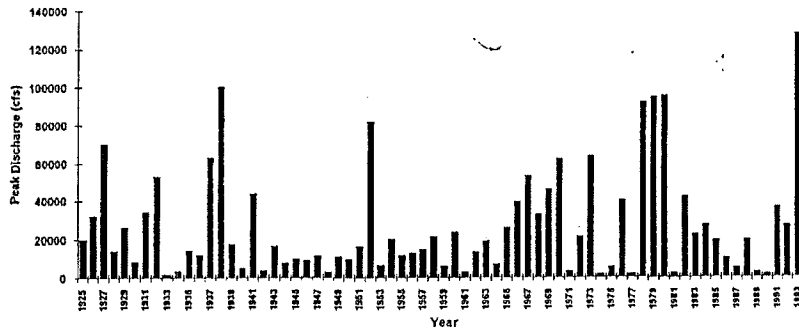
Figure 4c. Verde River Below Tangle Creek: Annual Maximum Flood Series 1925-1993
