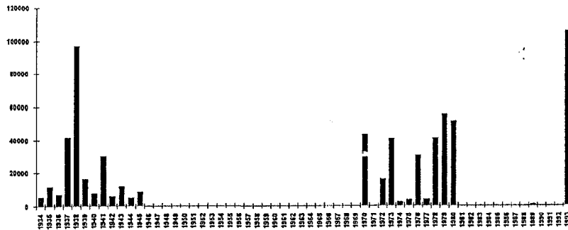
Figure 4b. Annual Maximum Flood Series: Verde River Near (1934-1945, 1989-1993) and Below (1970-1980) Camp Verde
