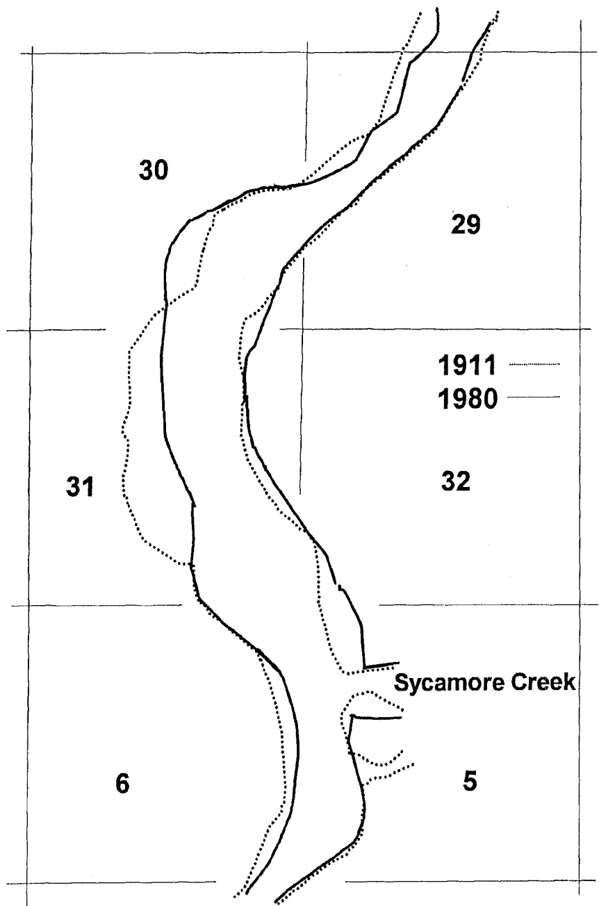
Figure 5d. Net changes in the position and width of the flood channel of the lower Verde River near Sycamore Creek between 1911 and 1980.
