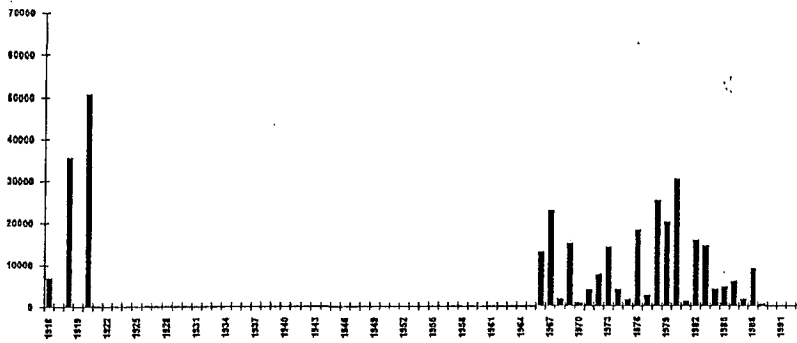
Figure 4a. Annual Maximum Flood Series: Verde River at Clarkdale
