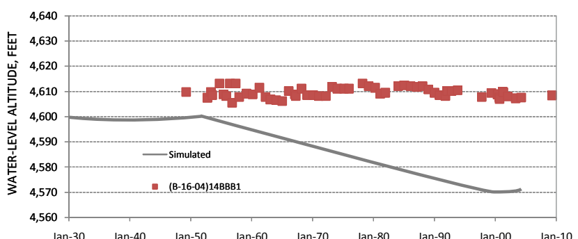
Figure 26. Hydrographs of simulated and observed water levels at selected wells in the Big Chino sub-basin.
