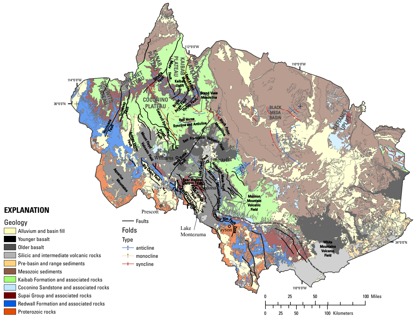
Figure 8. Surficial geology in the Northern Arizona Regional Groundwater-Flow Model study area. Geology modified from Utah State University (2004). Faults and folds modified from Ewing and others (1994), Reynolds (1988), DeWitt and others (2005), Blasch and others (2006), and Bills and others (2007).
