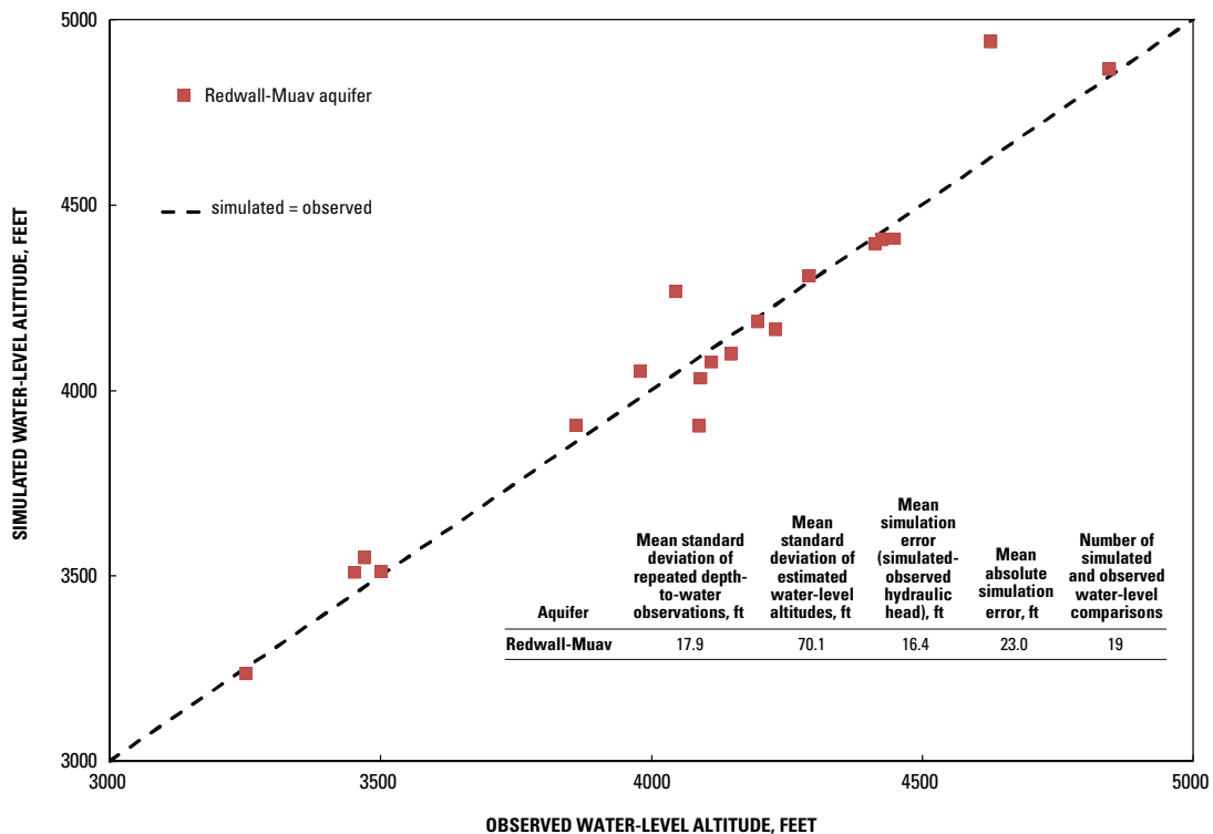
Figure 22. Simulated and observed predevelopment hydraulic head at wells in the Coconino Plateau basin and adjacent area.
