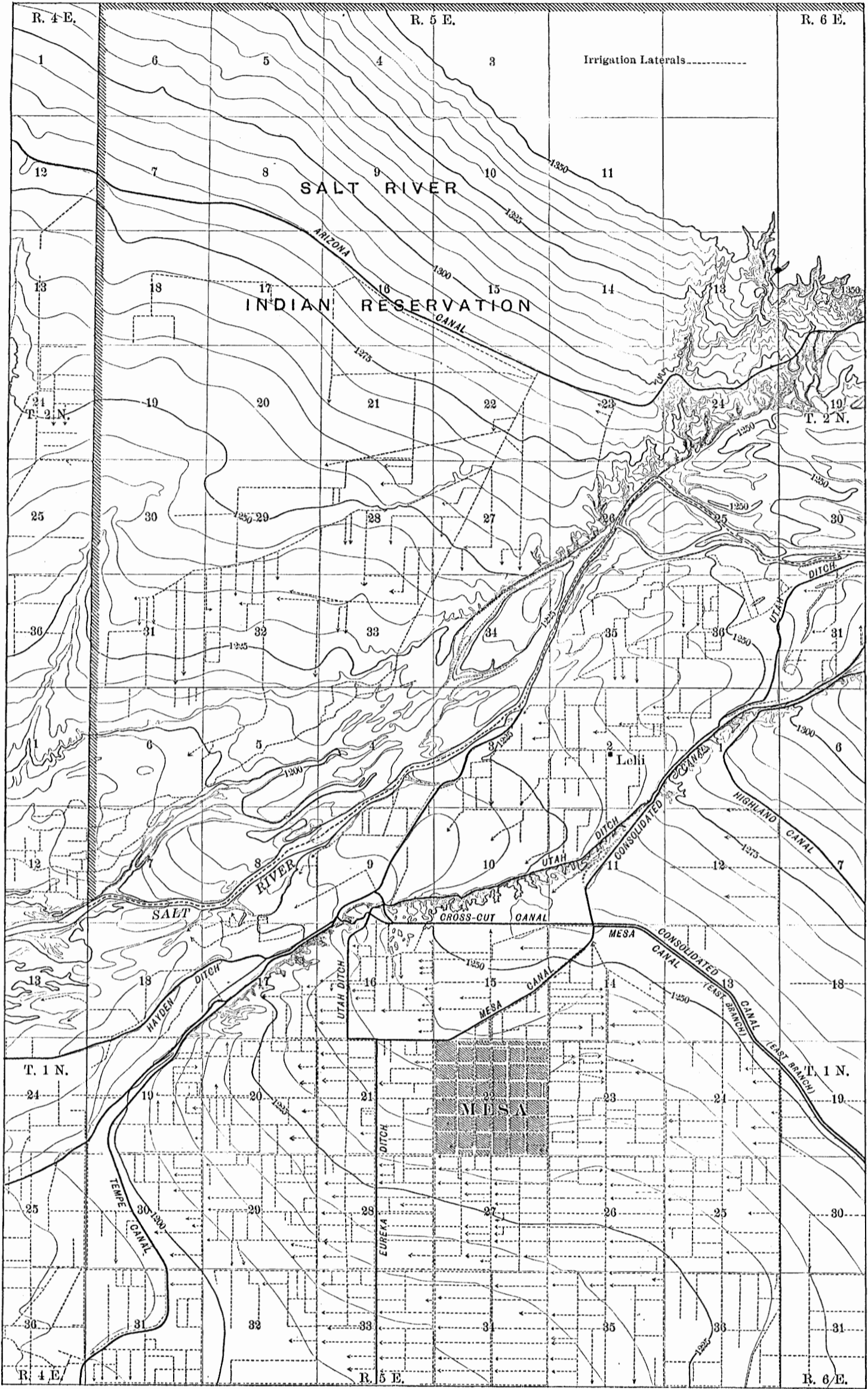
TOPOGRAPHIC MAP OF VICINITY OF MESA, ARIZ., SHOWING IRRIGATION CANALS AND DISTRIBUTION OF WATER BY LATERAL DITCHES.
