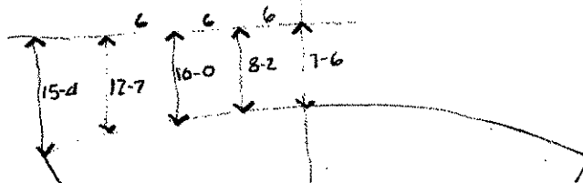
AFT BULKHD.
