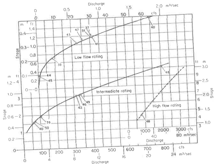
Figure 4-11 A simple stage-discharge relation.
