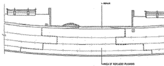
STARBOARD REPAIR
