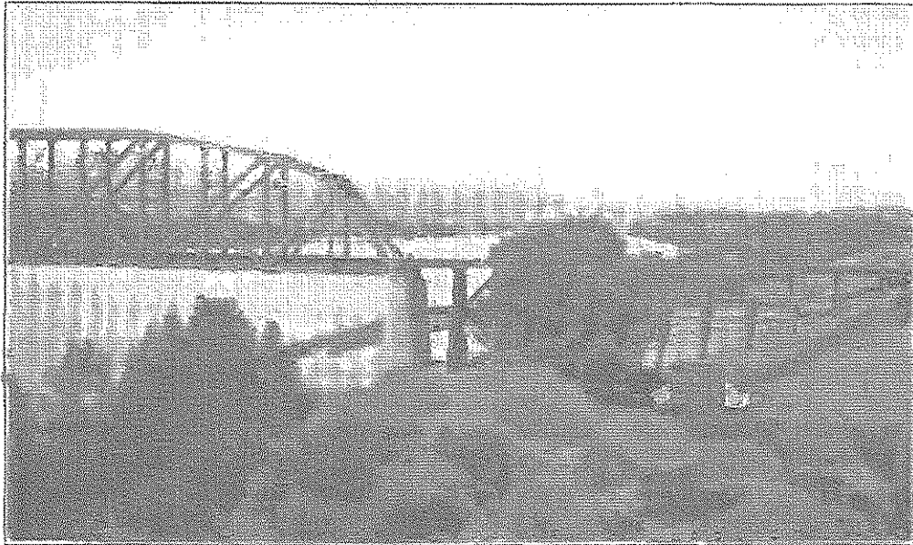
A. COLORADO RIVER AT PARKER. Showing bridge of Atchison, Topeka & Santa Fe Railway.
