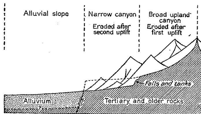
FIGURE 5.—Diagram showing production of falls and tanks by renewed uplift of eroded fault-block mountains.
