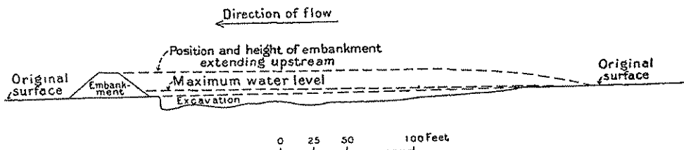
FIGURE 9.—Profile through typical Papago represo.
