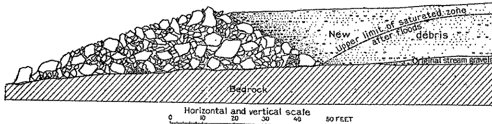
FIGURE 13.—Diagram showing rock-fill dam for an artificial reservoir.
