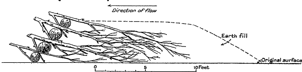
FIGURE 11.—Diagram showing the use of logs and brush for diversion dams and spillways.
