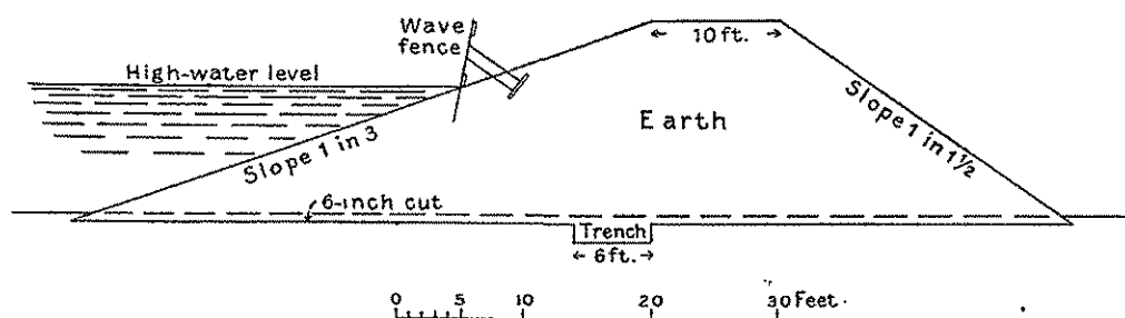
FIGURE 10.—Cross section of earth dam.
