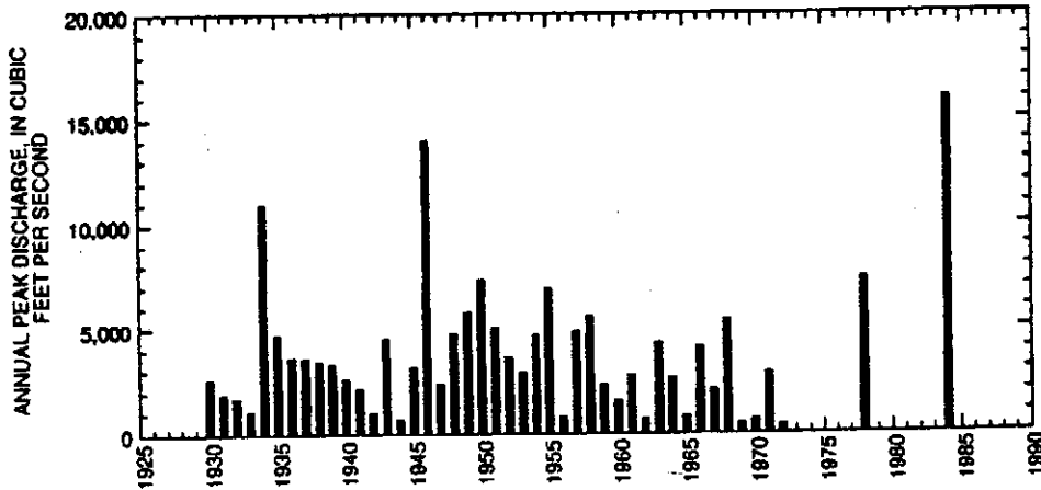
Figure 4: Annual Discharge Data for Sonoita Creek near Patagonia
