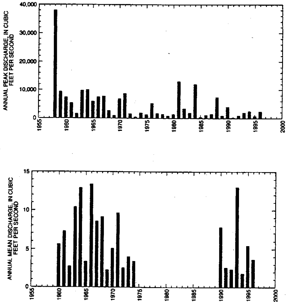
Figure 7: Annual Peak and Mean Discharge Data for Cienega Creek at Vail
