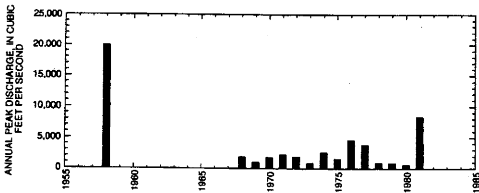
Figure 8: Annual Peak Discharge Data for Cienega Creek at Interstate-10
