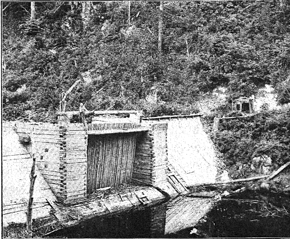
1. SPLASH DAM ON LITTLE RIVER, TENNESSEE.
