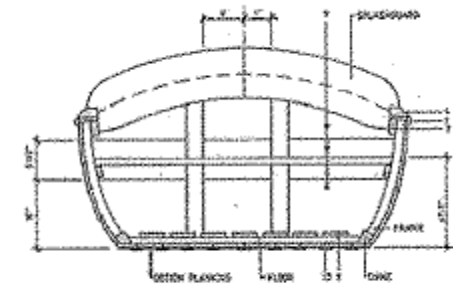
MID-SHIPS SECTION LOOKING FORWARD
